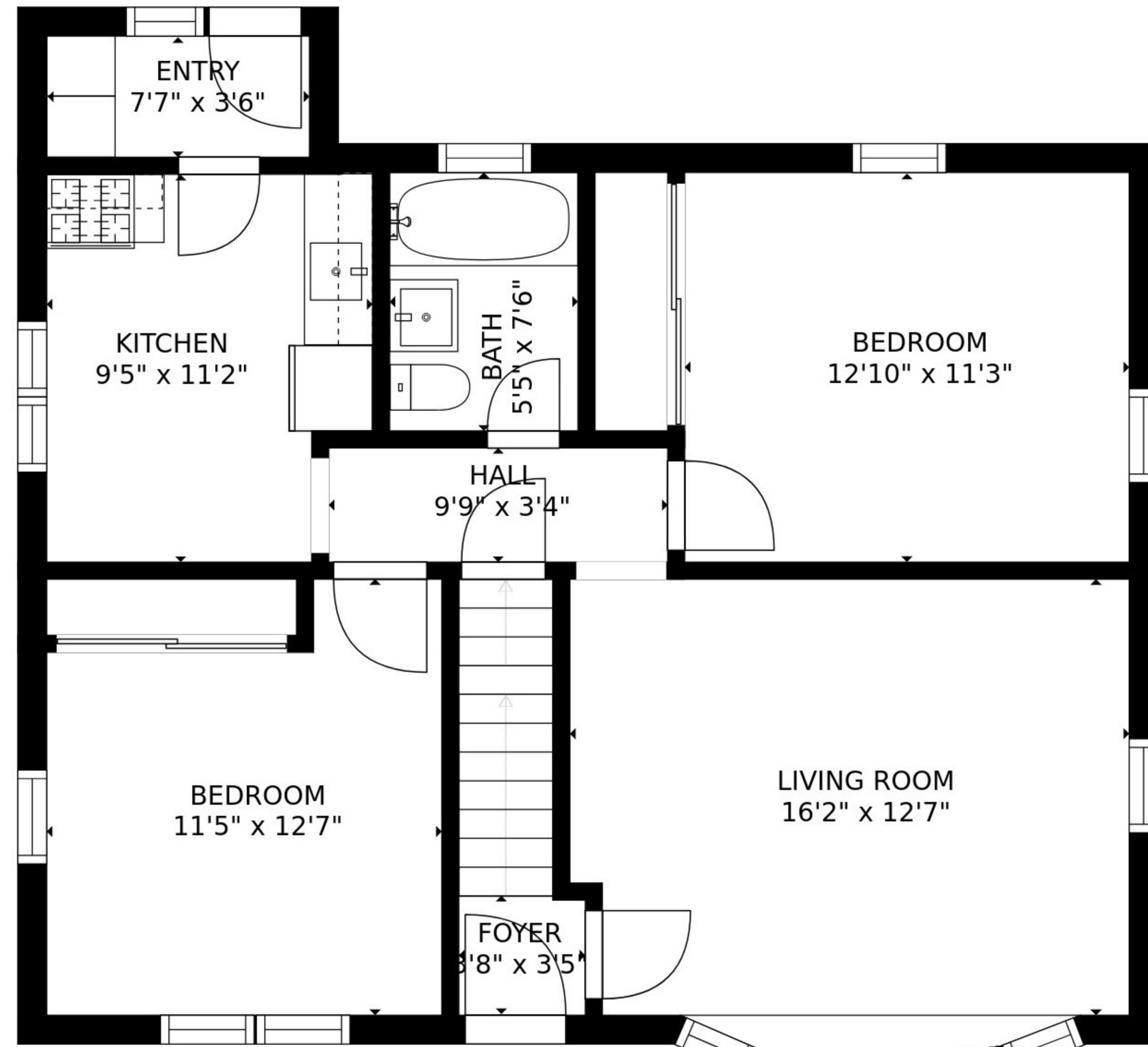
FIRST FLOOR
