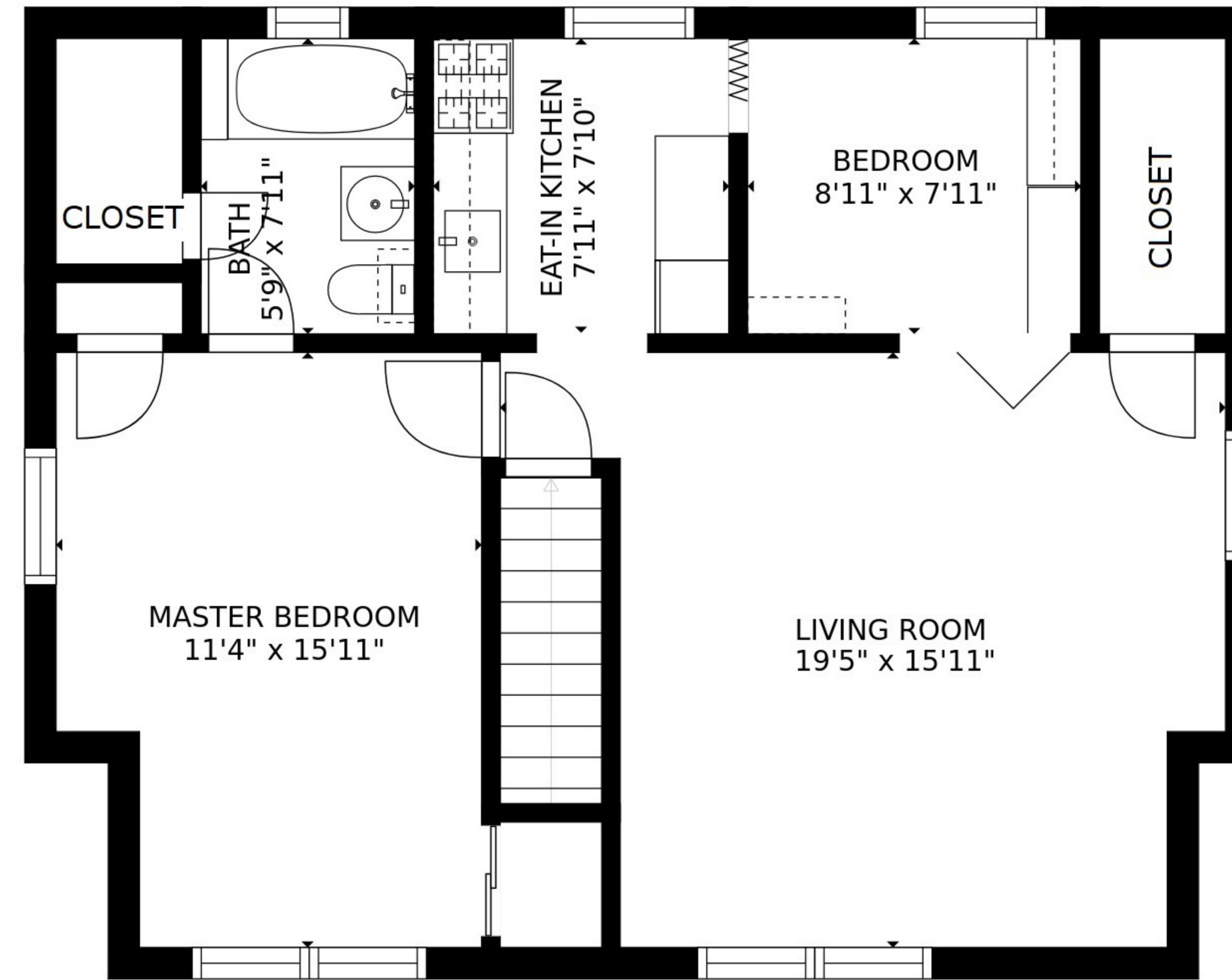
SECOND FLOOR
