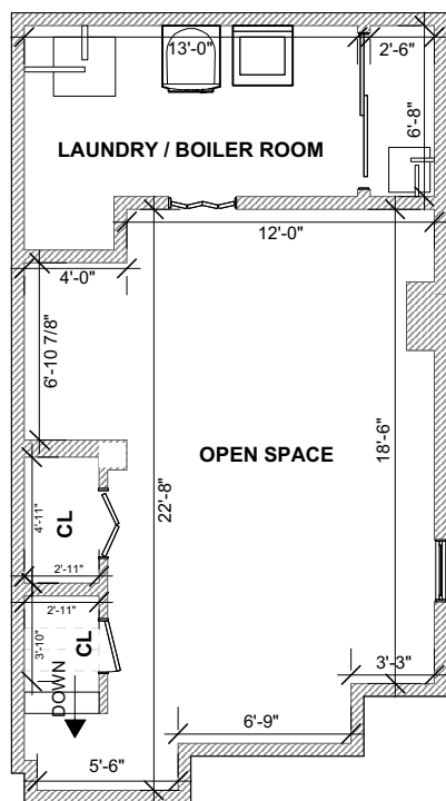
BASMENT TOTAL SQ. FT. 497.66
