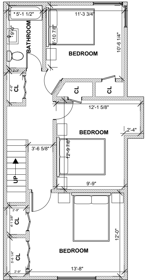
SECOND FLOOR TOTAL SQ. FT. 729.25
